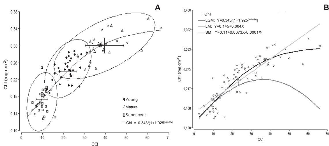
Figure 2. A) Relationship between total leaf chlorophyll concentration ( Chl \text{mg cm}^{-2} ) and meter readings ( CCI ) from Origanum vulgare ssp. hirtum leaves with standard deviations. Each subset of readings represents different leaf ages delimited by prediction ellipse. B) Logistic model (LGM) compared with linear (LM) and second-order polynomial models (SM).
